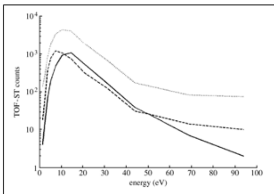
Energy distribution for ions (Michael, M. et al. 2005)
