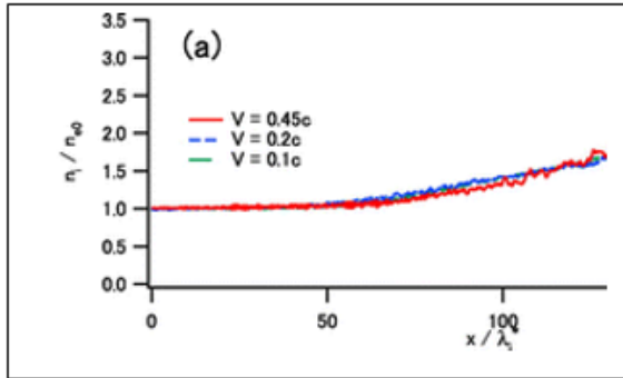
The ratio of ion density to electron density in unmagnetized plasma, which is around one (Kato, and Takabe, 2008)
