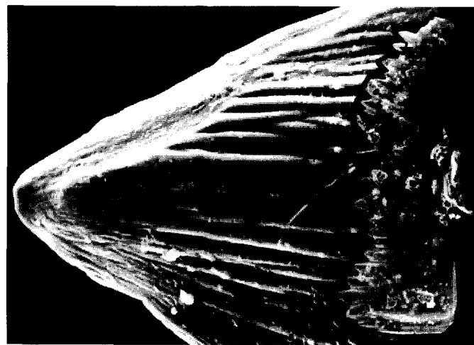
Fig. 6. Pa element of Ozarkodina from the Silurian of the Welsh Borders [whole element at right ( \times 42 ), close up to left ( \times 1466 )]. A well-developed wear facet (see close up) formed by contact with the opposed element sharply truncates the original fibrous surface texture. The facet is covered with fine parallel striations which indicate that this element was used for shearing; the arrow (top right) indicates the orientation of shearing motion. The distinctive nature of this facet and its location, between denticles, preclude a post mortem origin. Conodonts lacked jaws, and it has yet to be established quite how they were able to control occlusion between elements to the level of precision suggested by the parallelism of such striations. Specimen X-1299, Natural History Museum, London, UK. Reproduced, with permission, from Ref. 35.
