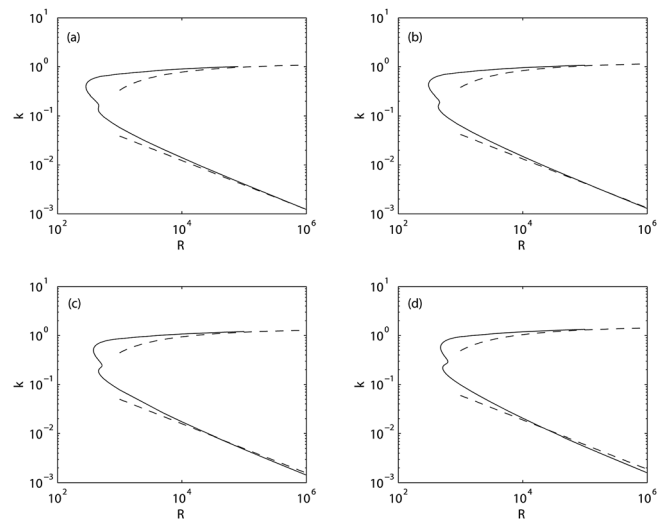
FIG. 2. Neutral-stability curves in terms of predicted wavenumber for T_s = 0, 0.05, 0.15, and 0.25 (a)–(d). Solid line: numerical, dashed line: asymptotic.
