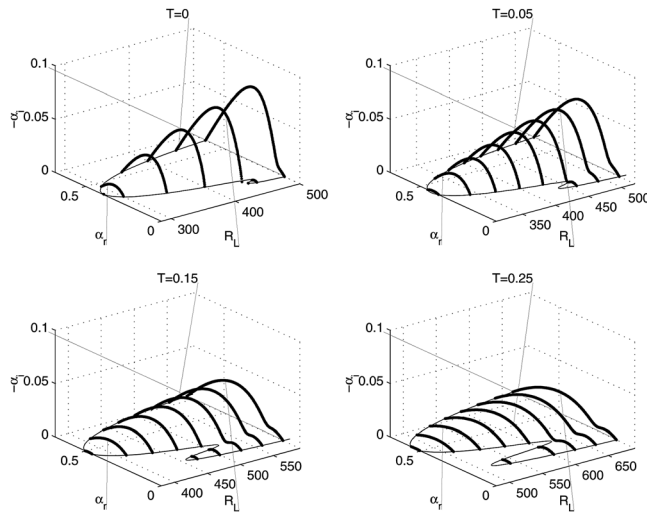
FIG. 6. Linear convective growth rates for stationary disturbances at various T_s at a fixed extent of 215 in R_L into the convectively unstable region.
