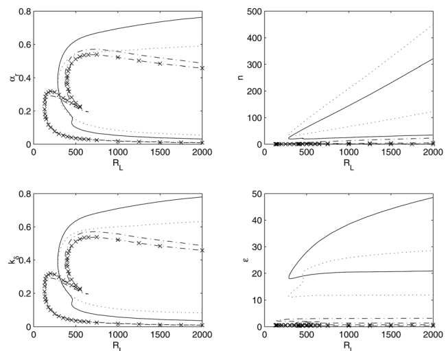
FIG. 13. Neutral-stability curves for traveling mode disturbances for T_s = 0 ; c = 0.8 “...”; c = 1 “-”; c = 5 “-.”; c = 20 “-x”.
