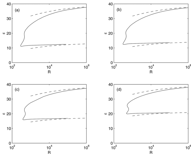
FIG. 3. Neutral-stability curves in terms of predicted waveangle for T_s = 0, 0.05, 0.15, and 0.25 (a)–(d). Solid line: numerical, dashed line: asymptotic.
