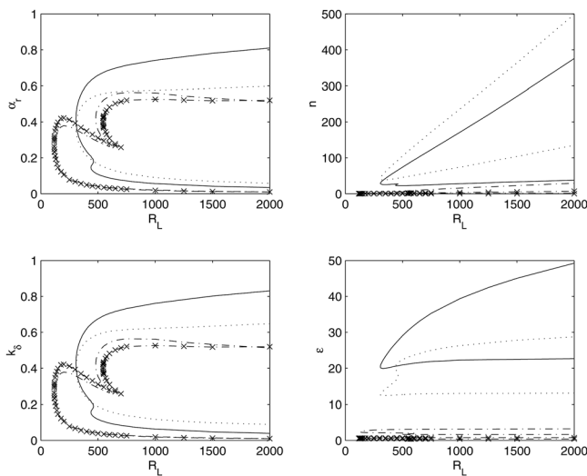
FIG. 14. Neutral-stability curves for traveling mode disturbances for T_s = 0.05 ; c = 0.8 “...”; c = 1 “—”; c = 5 “- -”; c = 20 “-x”.
