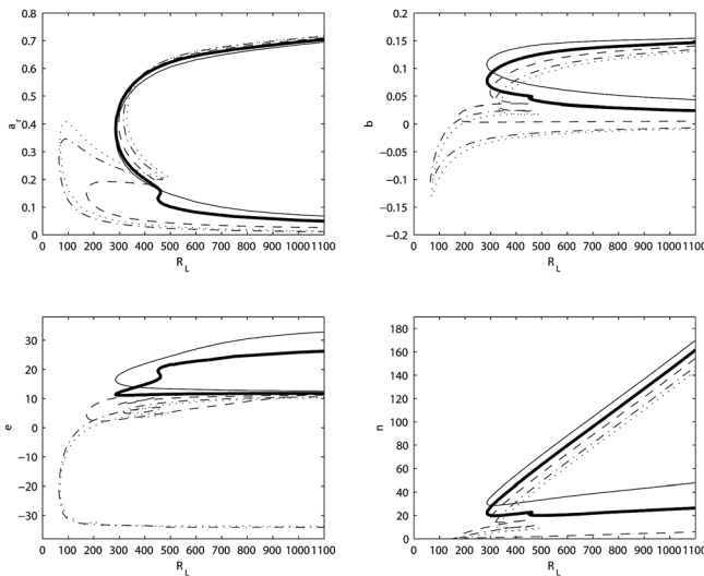
FIG. 9. Neutral-stability curves calculated in the rotating frame for \omega = 0 “—”; \omega = 4 “- -”; \omega = 7.9 “...”; \omega = 10 “- · - ·”; \omega = -5 “- - -” ( T_s = 0 ).
