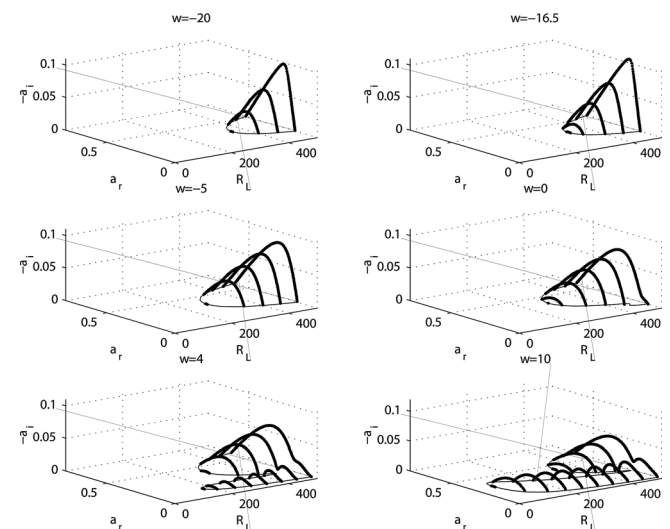
FIG. 11. Growth rates for T_s = 0 in the rotating frame for various \omega .
