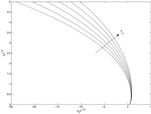
FIG. 7. Re-scaled leading-order wavenumber \bar{\gamma}_0 against the re-scaled frequency \bar{\omega}_0 shown for increasing axial flow T_s .
