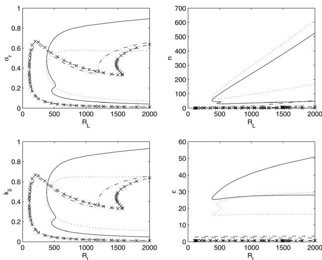
FIG. 15. Neutral-stability curves for traveling mode disturbances for T_s = 0.15 ; c = 0.8 “...”; c = 1 “—”; c = 5 “- -”; c = 20 “-x”.
