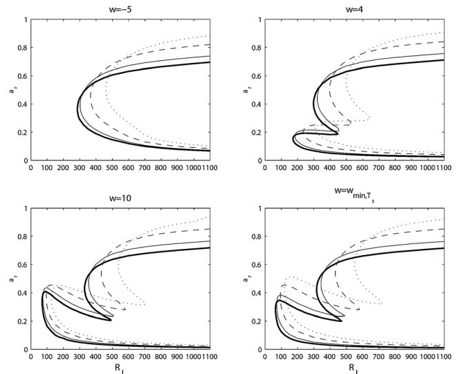
FIG. 10. Neutral-stability curves of traveling modes in the rotating frame for T_s = 0, 0.05, 0.15 , and 0.25 (left to right).
