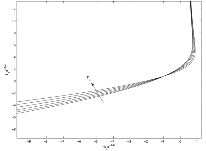
FIG. 8. Re-scaled first-order waveangle \bar{\phi}_1 against the re-scaled frequency \bar{\omega}_0 shown for increasing axial flow T_s .
