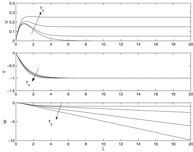
FIG. 1. Basic-flow profiles for T_s = 0, 0.05, 0.15, and 0.25 (arrow indicates direction of increasing T_s ).
