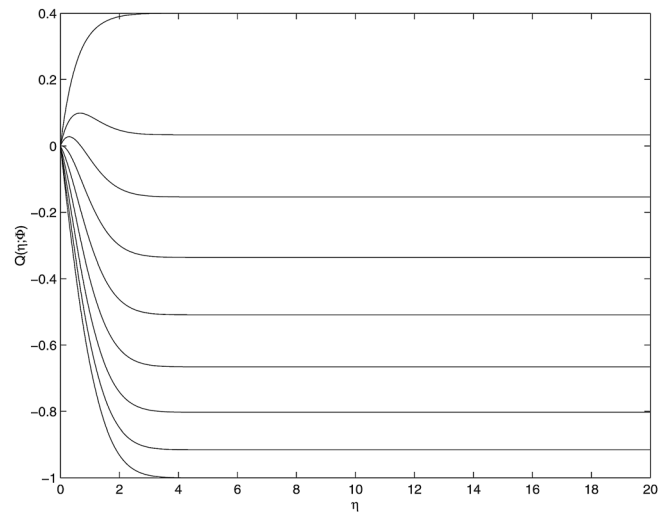
FIG. 5. The effective mean velocity profiles (in the rotating frame) for T_s = 0.40 at \Phi = 90^\circ - 0^\circ in increments of 10^\circ (bottom to top).
