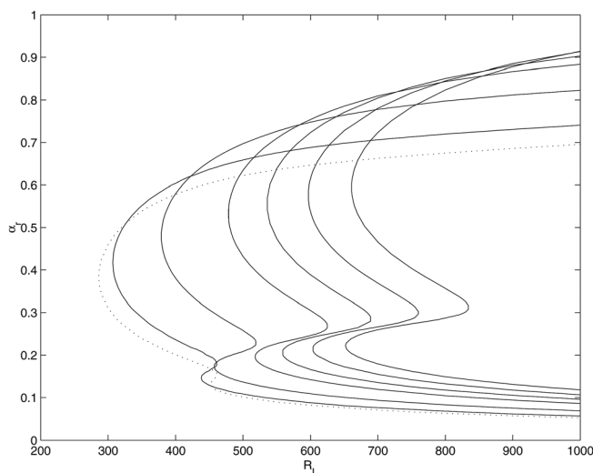
FIG. 4. Neutral-stability curves in the (\alpha_r, R_L) -plane for T_s = 0 (dotted line), 0.05, 0.15, 0.25, 0.30, 0.35, and 0.40 (left to right).
