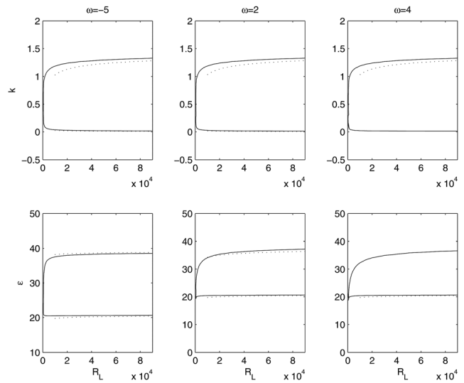
FIG. 12. Neutral-stability curves for T_s = 0.25 for traveling modes. Solid lines: numerical, dashed lines: asymptotic.
