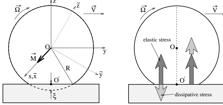
Fig. 1. – Sketch of the rolling sphere, the right figure shows the appearance of the friction momentum: in the front the elastic stress is enhanced by the dissipative stress, while in the rear it is diminished.
